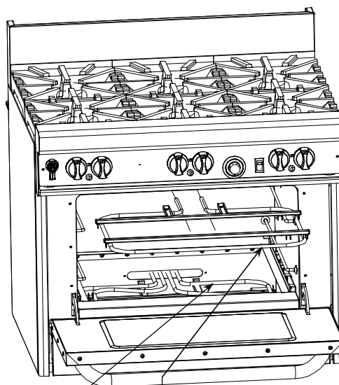
Top Element (Standard Oven) 208V P/N 1191621 240V P/N 1191622 480V P/N 1191625
