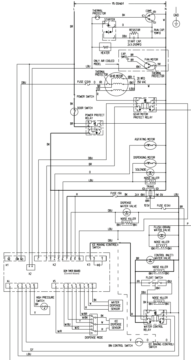
WIRING DIAGRAM
