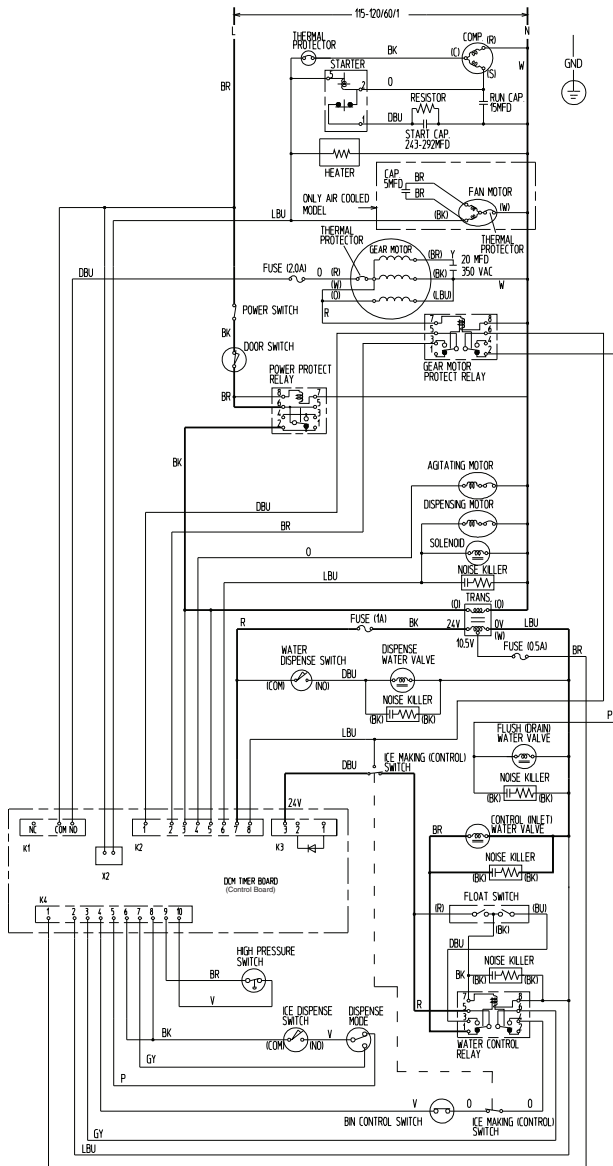
WIRING DIAGRAM
