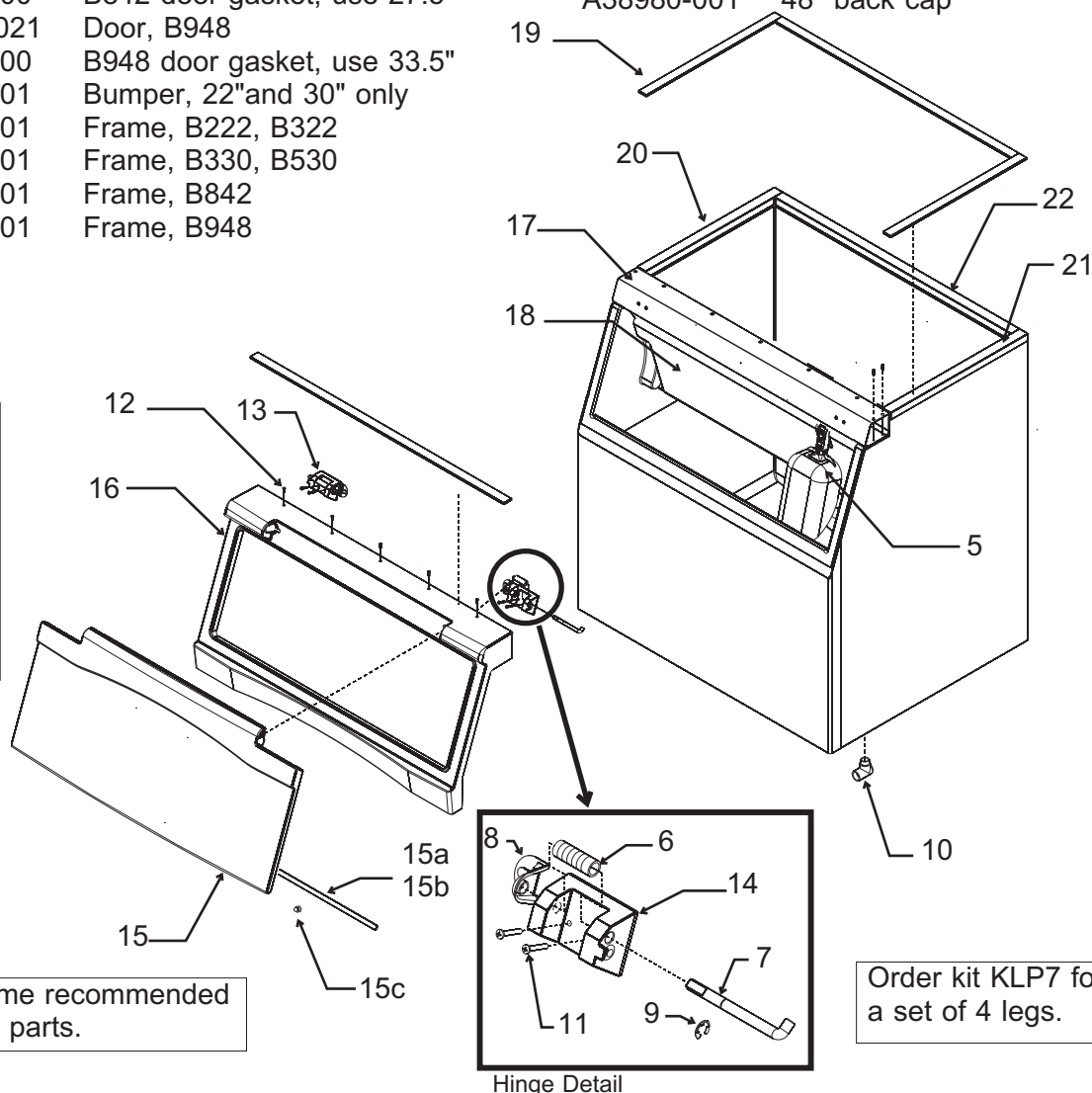
Hinge Detail
