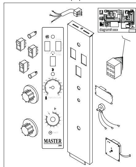
Controller Conversion Kit (6C)
