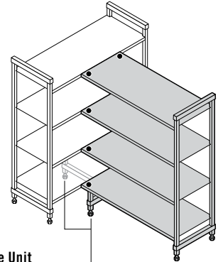
Starter + Add-On Unit With Shared Post
