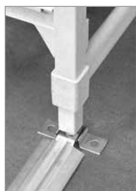
Hole diameter 3/8".
