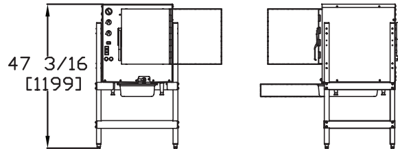
SINGLE XS ON 170944 STAND LOWEST SHELF WITHOUT CASTORS
